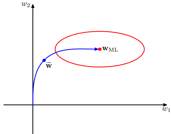
Figure 5.13 A schematic illustration of why early stopping can give similar results to weight decay in the case of a quadratic error function. The ellipse shows a contour of constant error, and w_{ML} denotes the minimum of the error function. If the weight vector starts at the origin and moves according to the local negative gradient direction, then it will follow the path shown by the curve. By stopping training early, a weight vector \tilde{w} is found that is qualitatively similar to that obtained with a simple weight-decay regularizer and training to the minimum of the regularized error, as can be seen by comparing with Figure 3.15.
