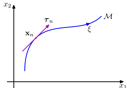
Figure 5.15 Illustration of a two-dimensional input space showing the effect of a continuous transformation on a particular input vector \mathbf{x}_n . A one-dimensional transformation, parameterized by the continuous variable \xi , applied to \mathbf{x}_n causes it to sweep out a one-dimensional manifold \mathcal{M} . Locally, the effect of the transformation can be approximated by the tangent vector \tau_n .
